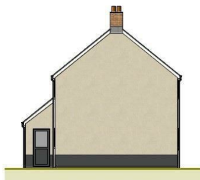
South East Elevation. Scale 1:100
